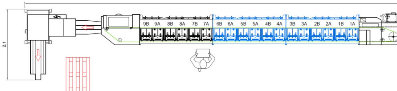
Smyth gatherer mod. P12 with 9 (18) stations + stacker
